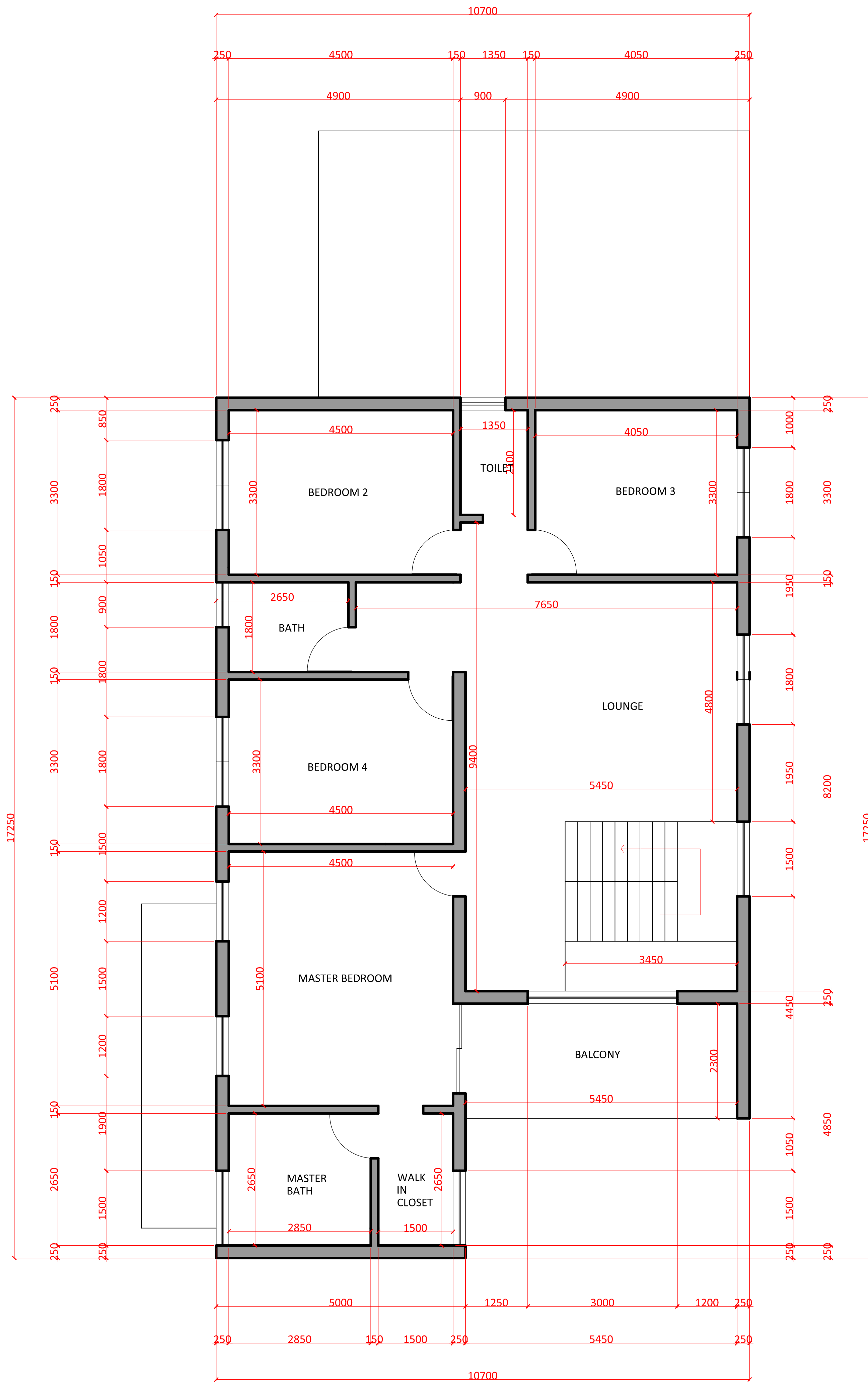
A' FIRST FLOOR LAYOUT PLAN @ FIVE BEDROOM RESIDENCE
