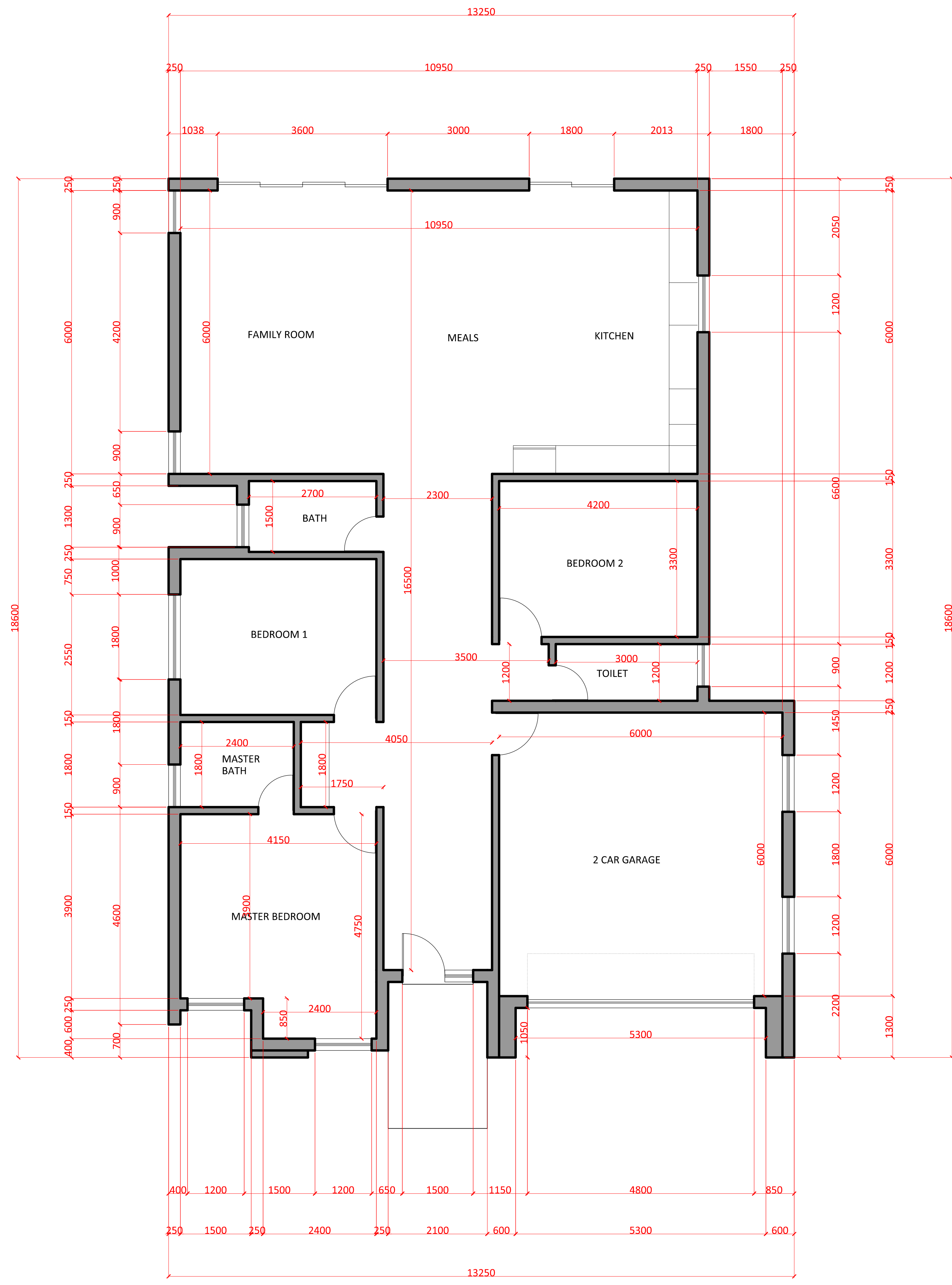
A' LAYOUT PLAN @ THREE BEDROOM RESIDENCE
